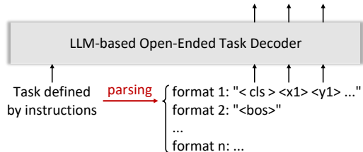
Figure 4: Illustration of the “output-format-as-query” decoding process. “ \langle \text{cls} \rangle \langle x1 \rangle \langle y1 \rangle \dots ” denote the queries of the object’s class index and boundary points, and “ \langle \text{bos} \rangle ” denotes the beginning of string.
